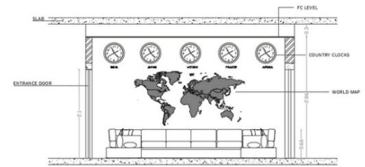
RECEPTION WALL ELEVATION
