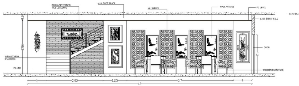
INDIAN STYLE WALL ELEVATION
