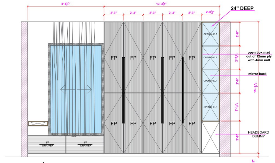
M.BED ROOM WARDROBE
