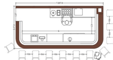
BAR COUNTER PLAN
