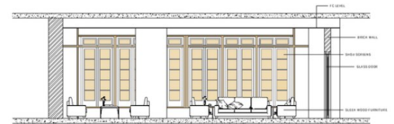
JAPANESE STYLE WALL ELEVATION
