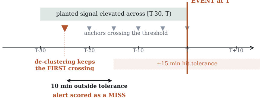
Figure 4 — A signal leading by more than the tolerance never scores a hit ILLUSTRATIVE SCHEMATIC — contains no measured values; the bug it depicts is quantified in §7.
