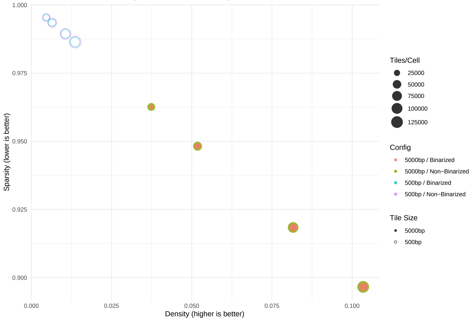
Binsize Tradeoff: 5000bp Non-Binarized is Optimal
