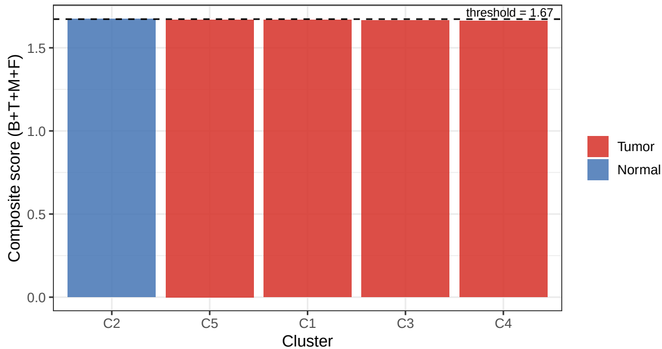
lowseq_489: Immune/stromal composite score per cluster
