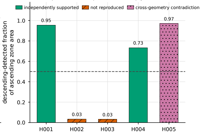
Reproduction is spatial and sharply selective
