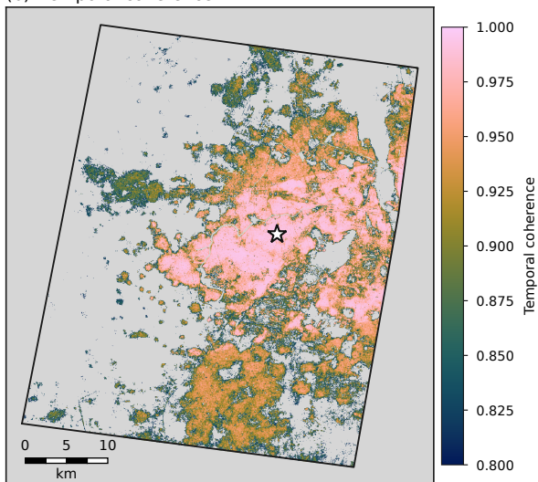
(b) Temporal coherence
