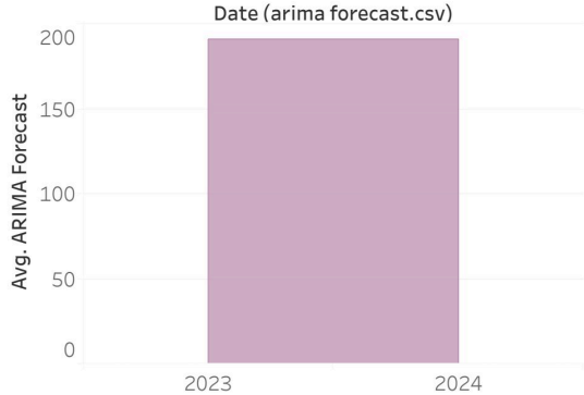
Arima ForeCast
