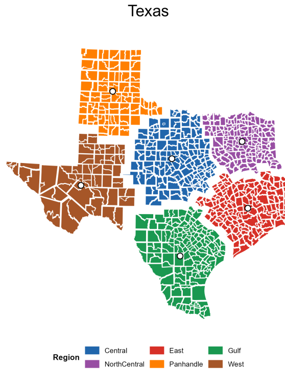
Figure 5: Texas county subdivisions after formula-derived displacement and documented display offsets. The layout demonstrates the larger-unit regime identified in Table 1.
