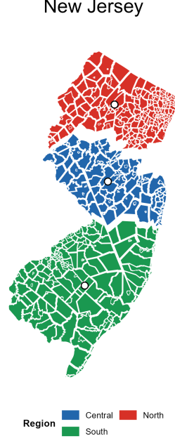
Figure 2: Exploded-view map of New Jersey municipalities ( n = 564 ) using the calibrated displacement values and documented display offsets. North, Central, and South regions are separated by the regional displacement term while each municipality’s internal geometry is preserved exactly. The display offsets are stored in paper/outputs/tables/nj_drag.offsets.csv .
