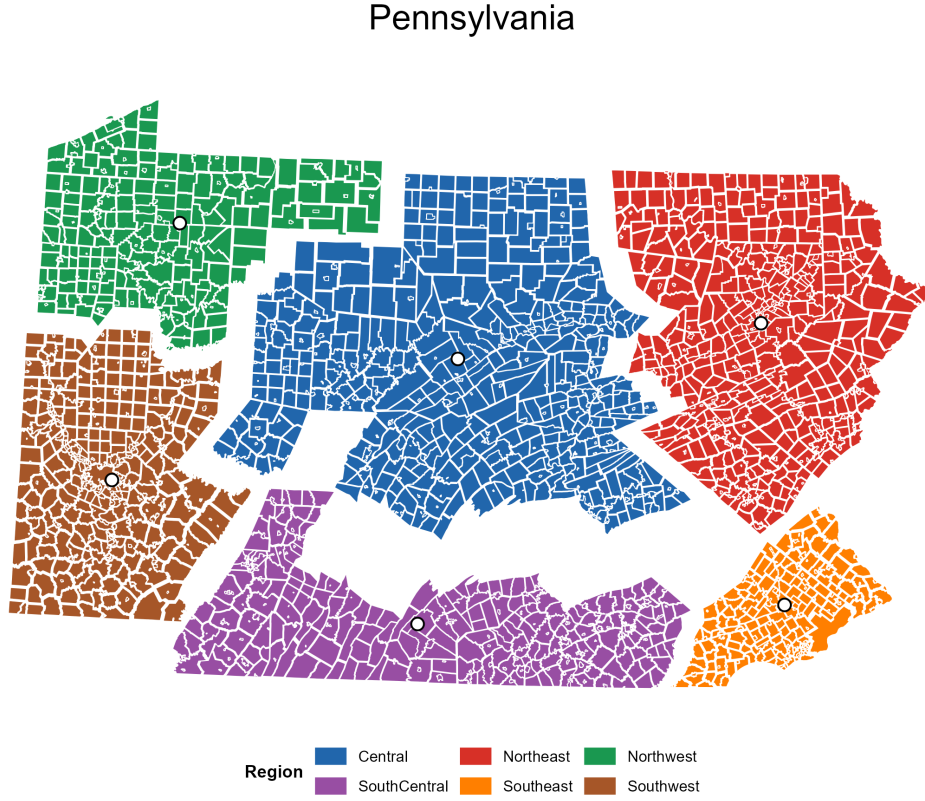
Figure 3: Pennsylvania municipalities ( n = 2,572 ) after formula-derived displacement ( \alpha_r = 20,174 m, \alpha_l = 12,447 m, p = 1.25 ) and documented region-level display offsets. The offsets are rigid translations recorded in paper/outputs/tables/pa_drag_offsets.csv ; they improve figure composition without changing any municipality’s shape, area, or within-region relative arrangement.
