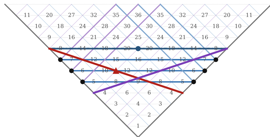
(b) X-Triangle: Ordinary Multiplication Table
