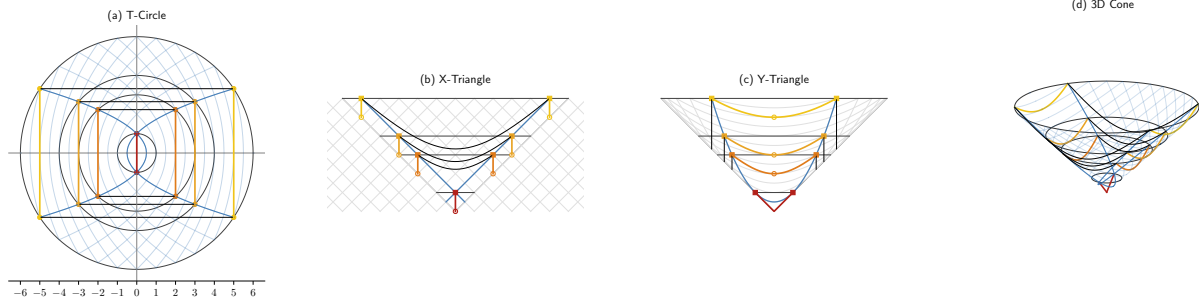
FIGURE 1. The four totient hyperbolas, four views of one object: (a) down the T axis, (b) down Y , (c) down X , (d) perspective. For each unit r \in \{1, 5, 7, 11\} the colored arc is the Paper-A hyperbolic section X = (r-1)/2 (yellow r = 11 to red r = 1 , degenerate), running from the open-circle vertex ((r-1)/2, 0, (r-1)/2) to the unit-shell squares (\pm(r-1)/2, \pm\sqrt{r}, (r+1)/2) on the landing circles T = (r+1)/2 (thin gray); black connectors join the shell points at constant Y = \sqrt{r} . The vertices X \in \{0, 2, 3, 5\} and the radii T \in \{1, 3, 4, 6\} square to QR(12) = \{0, 1, 4, 9\} \pmod{12} , the two bijections of Proposition 4.1.
