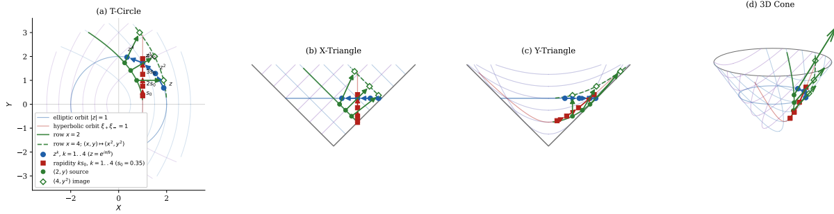
FIGURE 2. Eigen-coordinate power maps, four views of one object. Blue: elliptic circle |z| = 1 with the angle-multiplying markers z, z^2, z^3, z^4 for z = e^{i\pi/9} ; the flow z \mapsto e^{i\omega t}z becomes z \mapsto z^n on the orbit. Red: hyperbolic branch \xi_+\xi_- = 1 with rapidity markers s_0, 2s_0, 3s_0, 4s_0 ( s_0 = 0.35 ), the dilation s \mapsto ns . Green: parabolic boundary — the coordinatewise square (x, y) \mapsto (x^2, y^2) sends the row x = 2 parabola (solid) to the row x = 4 parabola (dashed); no diagonal eigen-coordinate exists here (Proposition 7.1). The faint blue/purple background is the canonical row/column parabola mesh of the cone (Paper A).
