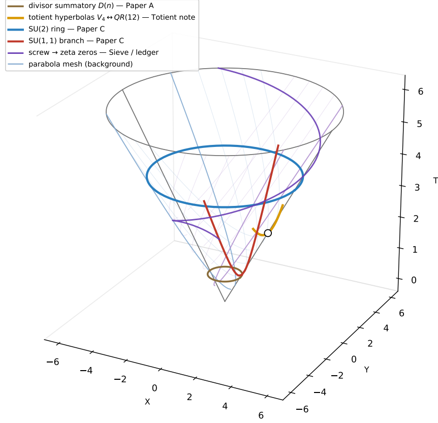
FIGURE 1. Schematic map of the program's readings on the one cone: the divisor-summatory base, the unit shell with its totient hyperbolas, a fixed- T SU(2) ring, a fixed- X SU(1,1) branch, and the screw curve running toward the analytic summit. Schematic only; see the cited papers for the exact statements.
