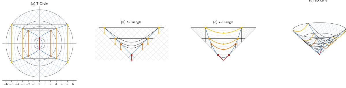
Figure 2: The mod-12 unit labels in the two-sided factor-cone coordinates. For each factor pair the full Cone contains the reflected lifts Y = \pm\sqrt{r} . The outer r = 11 pair is (11, 1) and (1, 11) on x + y = 12 . The geometric placement realizes the four labels but is not itself the multiplication law of U(12) .
