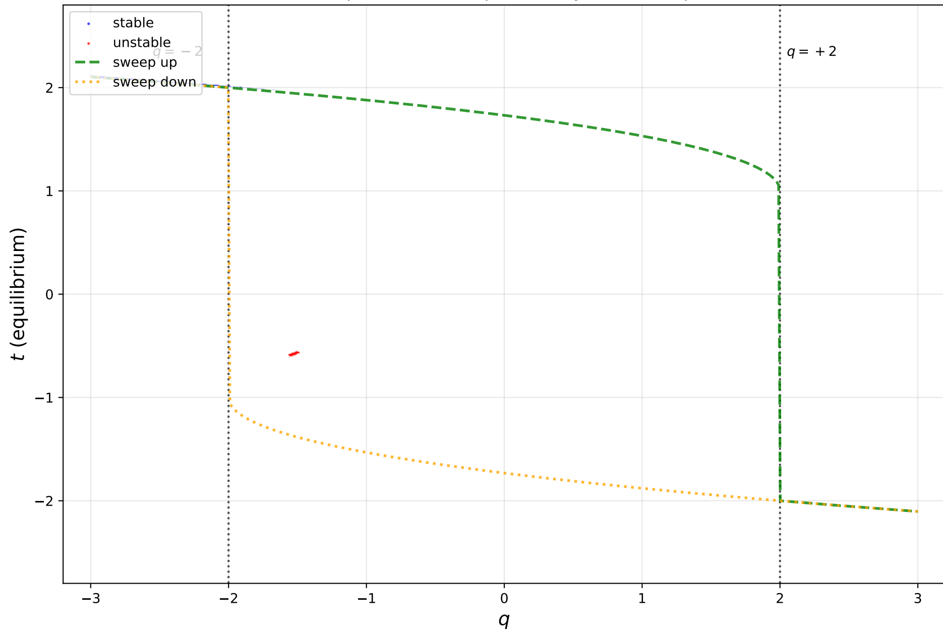
Cusp bifurcation at p = -3 : hysteresis loop
