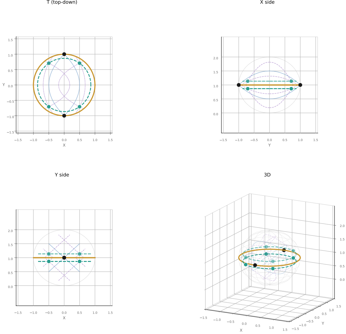
FIGURE 1. The bicone in the sphere: two copies of the Cone program's T -axis cone [4, 5], glued at the gold T_0 -circle, carrying su(2) \oplus su(2) \rightarrow so(4) . Four views: T (top-down, the T_0 -circle), X and Y sides, and 3D.
