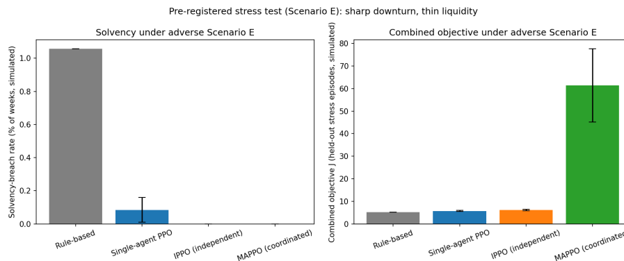
Figure 7: stress-test summary
