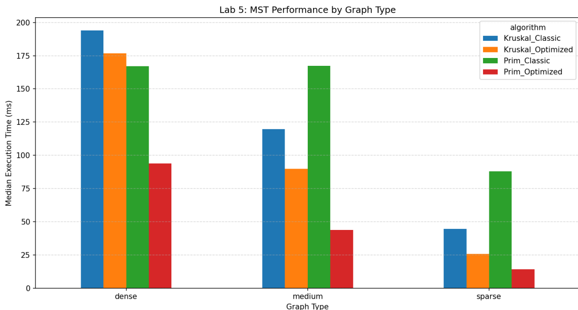
Figure 2.2 – Figure 2.2 – MST performance by graph type
