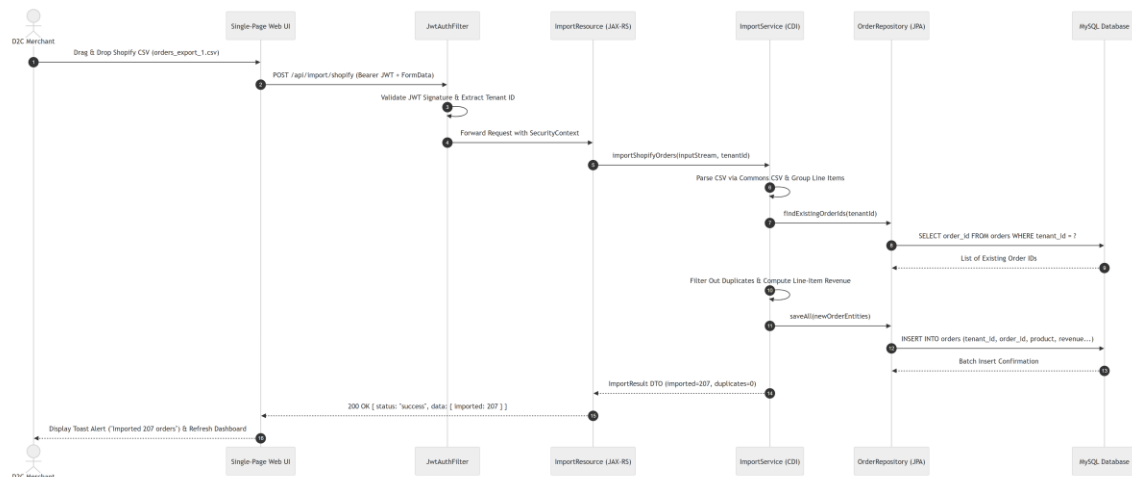
3.4 Sequence Diagram (CSV Ingestion Execution Flow)
