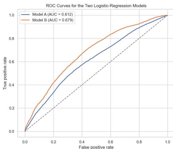
Figure 11: ROC curves comparing the athlete-level logistic regression model against the extended model that includes country.
