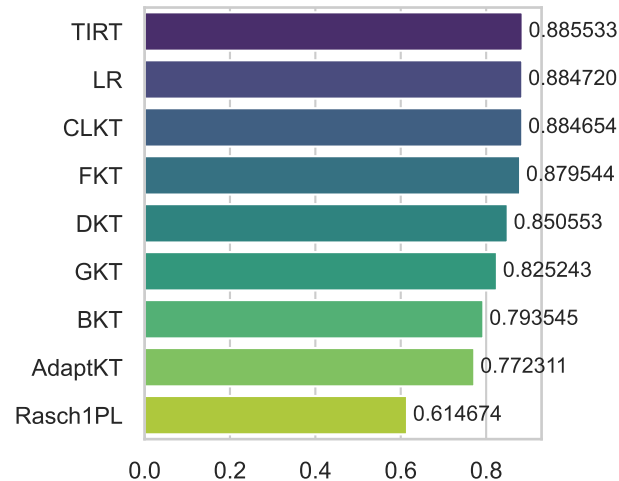
Average Precision (↑)
