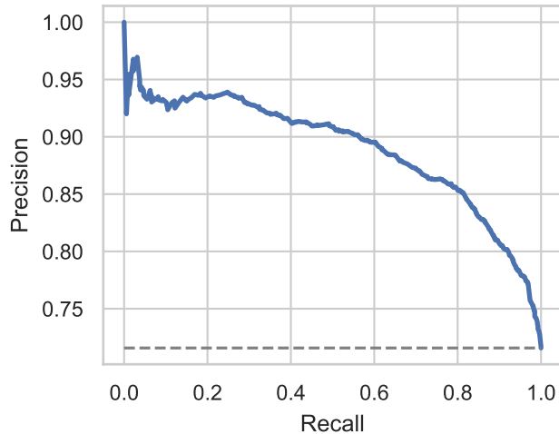
PR (AP=0.8895)
