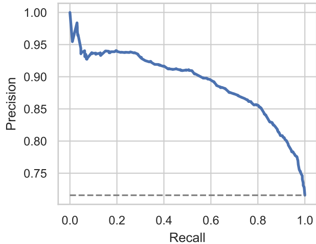
PR (AP=0.8912)
