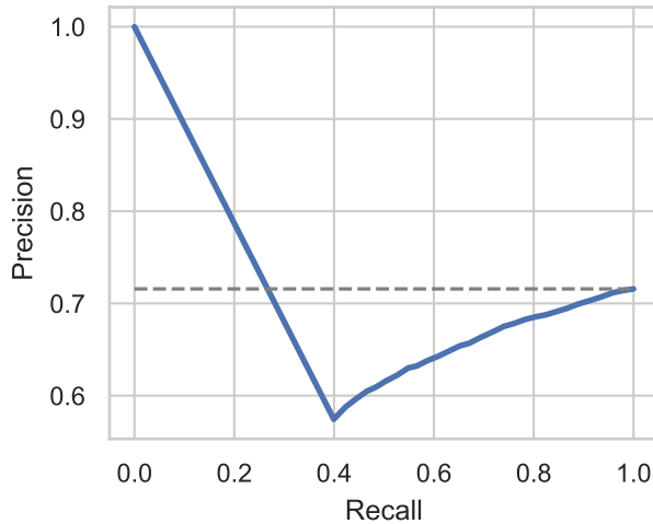
PR (AP=0.6269)
