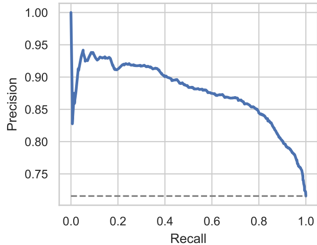
PR (AP=0.8772)
