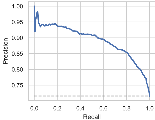
PR (AP=0.8906)
