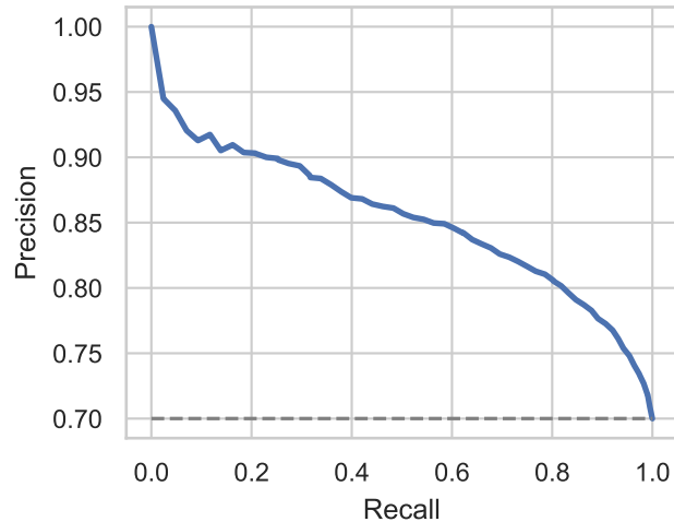
PR (AP=0.8506)
