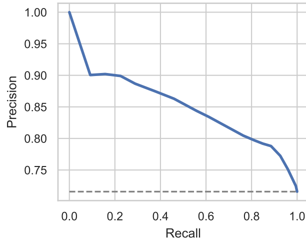
PR (AP=0.8400)
