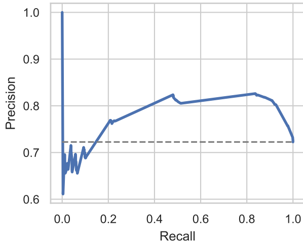
PR (AP=0.7966)
