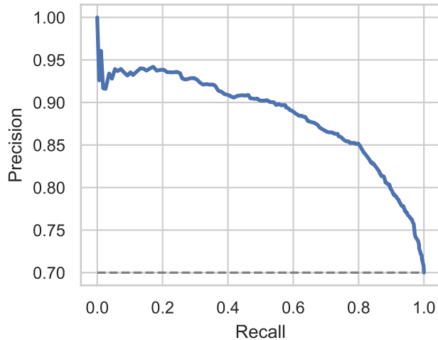
PR (AP=0.8847)
