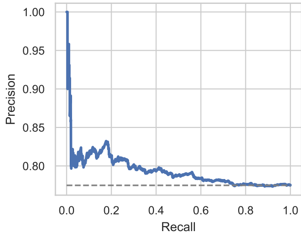
PR (AP=0.7942)
