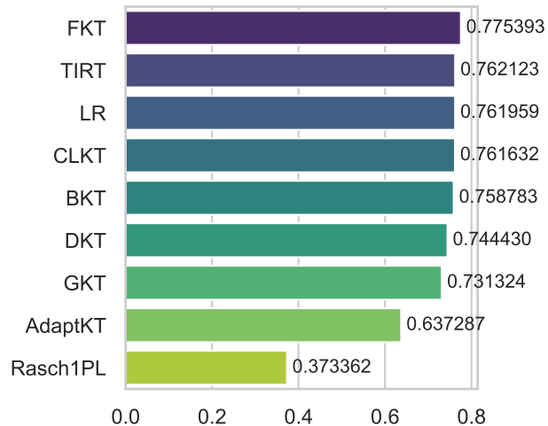
Log Loss (↓)
