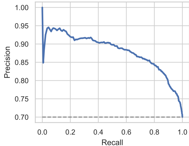
PR (AP=0.8795)
