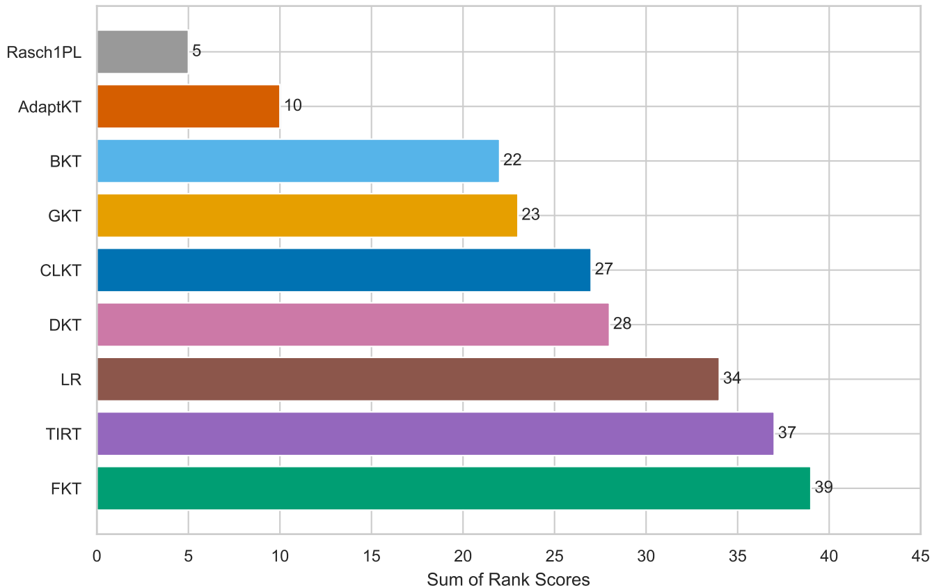
Sum of Rank Scores across Accuracy, ROC-AUC, AP, F1 Score, Log Loss
