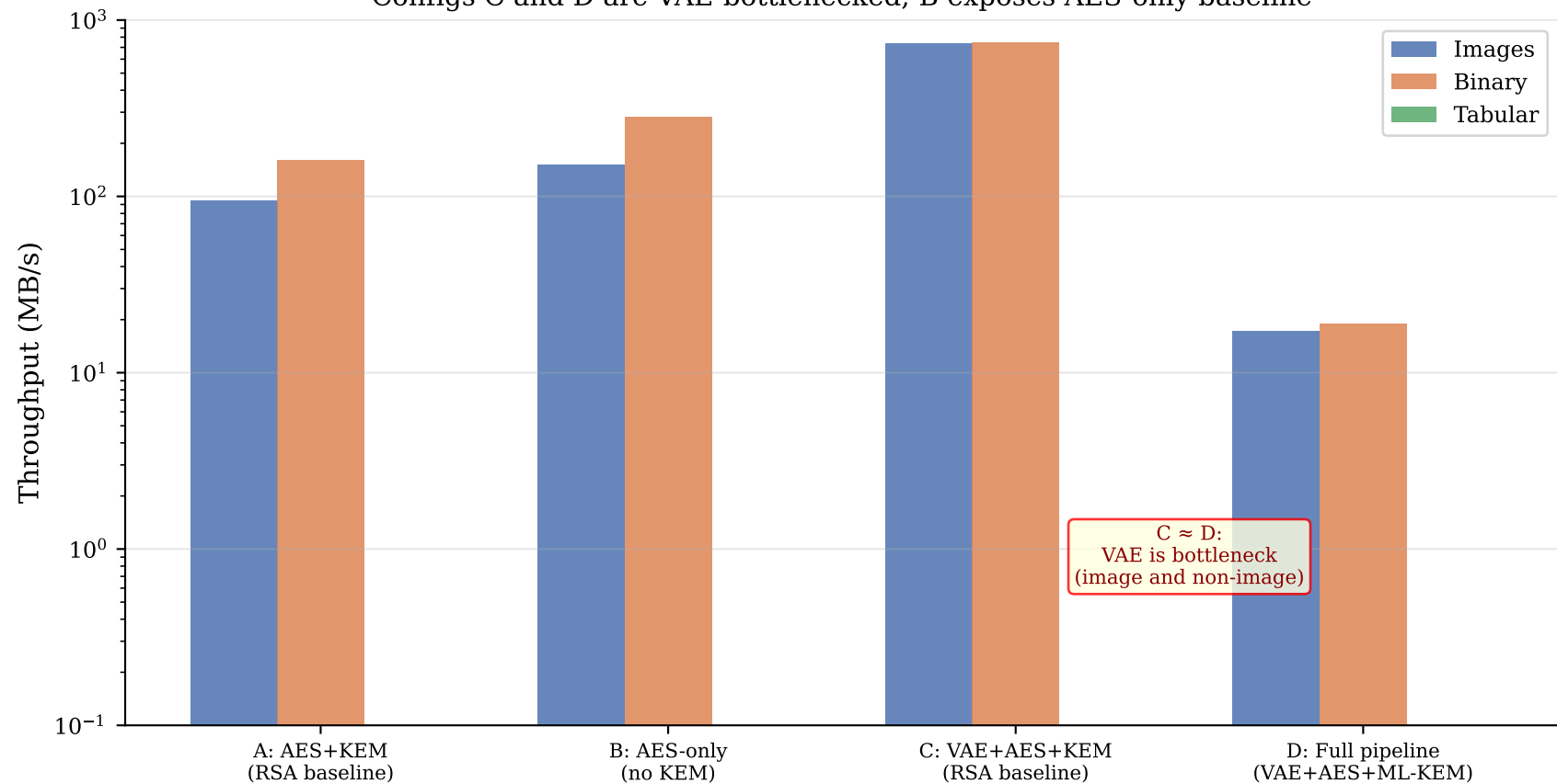
Figure 8 — Ablation study: throughput by configuration and file type Configs C and D are VAE-bottlenecked; B exposes AES-only baseline
