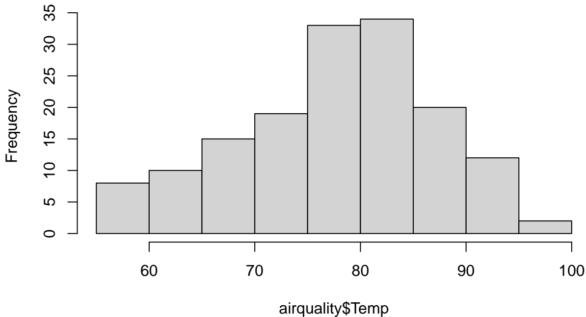
Histogram of airquality$Temp
