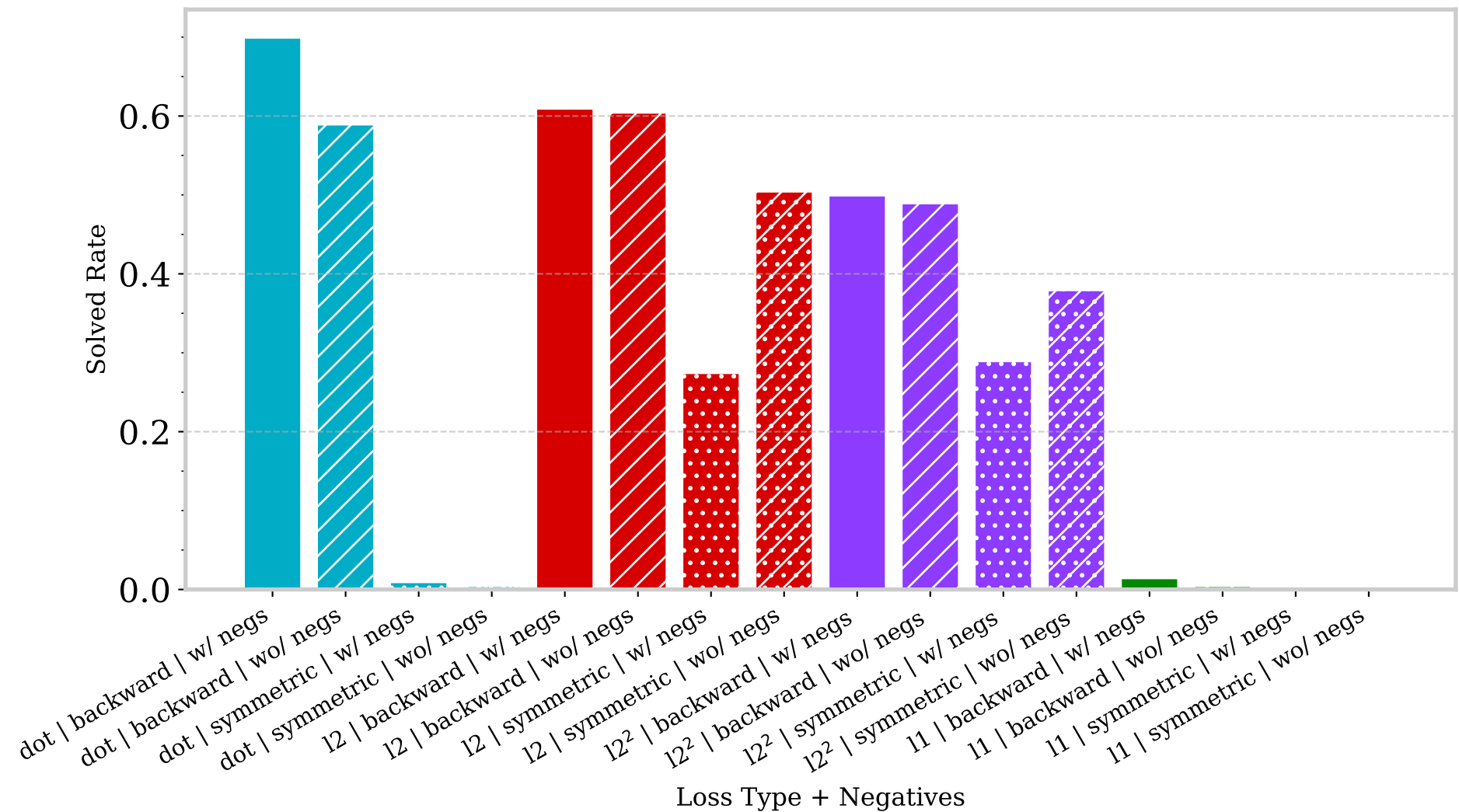
Final Solved Rate (1M training steps)
