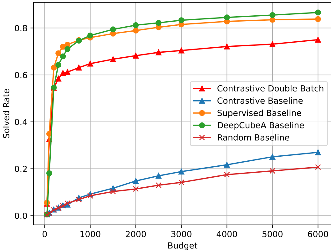
Sokoban Solved Rate vs. Budget
