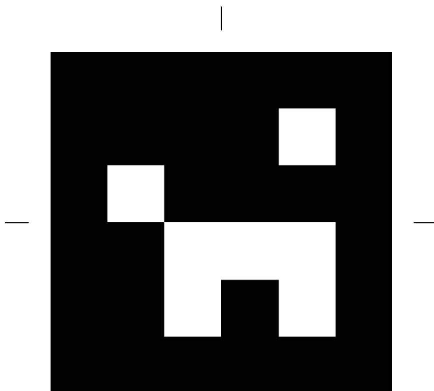
ArUco DICT_4X4_50 id 36 — 90 mm across (incl. black border); ticks mark the centre axes
