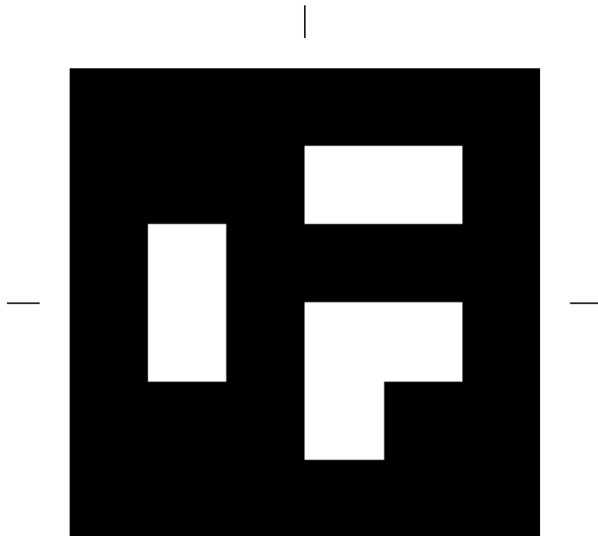
ArUco DICT_4X4_50 id 43 — 90 mm across (incl. black border); ticks mark the centre axes
