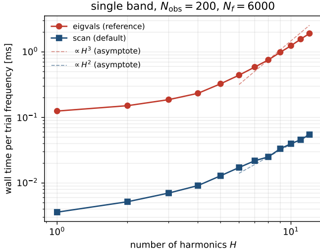
FIG. 1.— Wall time per trial frequency versus the number of harmonics H for the default scan+polish maximiser ( method='scan' , blue) and the reference polynomial-root implementation ( method='eigvals' , red), timed on identical well-conditioned single-band data ( N_{\text{obs}} = 200 , N_f = 6000 ). The default path is a measured factor of 25–35 faster across all H . At low H both paths are dominated by the shared \mathcal{O}(HN_f \log HN_f) NFFT summations and rise only mildly with H ; by H \gtrsim 8 the per-frequency maximiser takes over, and the reference cost steepens toward its \mathcal{O}(H^3) root-finding asymptote while the scan tracks \mathcal{O}(H^2) (dashed segments; the measured 8 \rightarrow 12 log–log slopes are \approx 2.3 and \approx 1.9 respectively).
