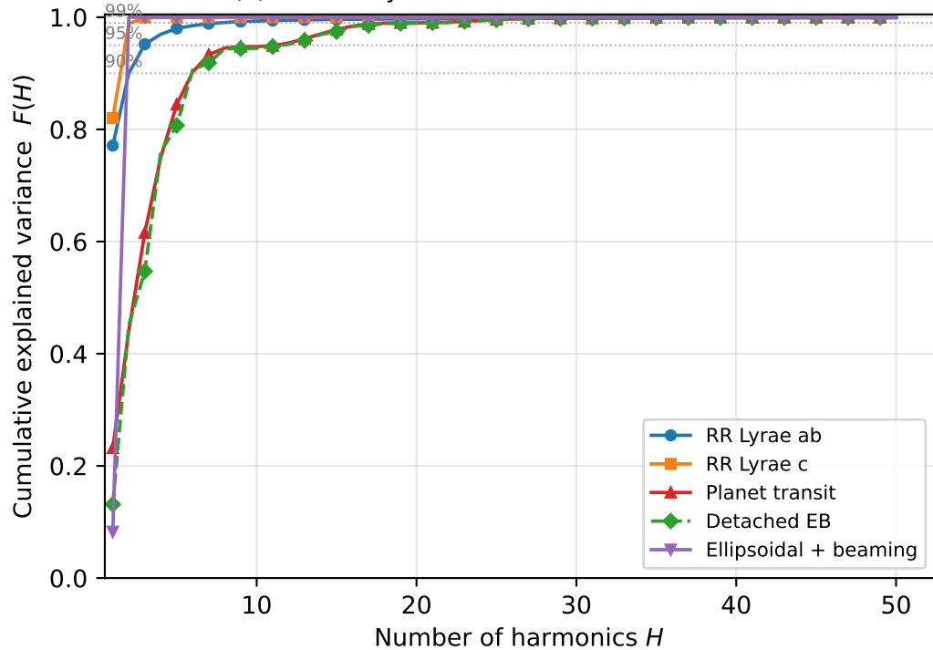
(a) L^2 fidelity of the H-truncated Fourier series
