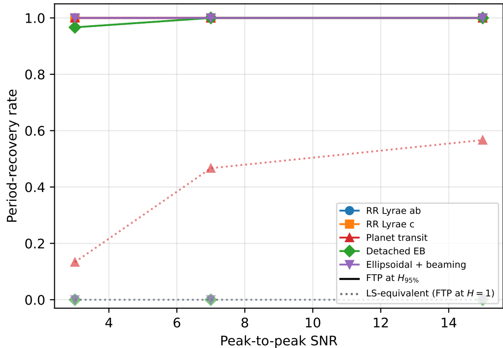
(b) Period recovery on synthetic LCs
