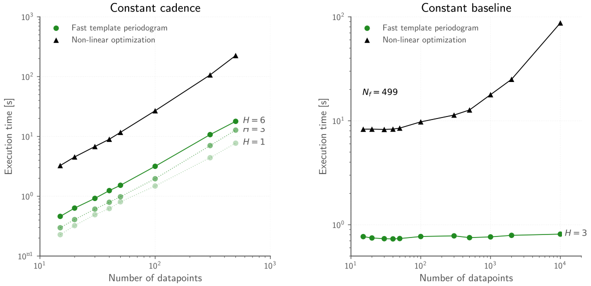
FIG. 6.— Computation time of FTP compared with alternative techniques that use non-linear optimization at each trial frequency. Left : timing for the case when N_f = 12N_{\text{obs}} , i.e. the cadence of the observations is constant. Right : timing for the case when N_f is fixed, i.e. the baseline of the observations are constant. Non-linear optimization techniques scale as \mathcal{O}(N_f N_{\text{obs}}) while the FTP scales as \mathcal{O}(HN_f \log HN_f + N_f H^3) , where H is the number of harmonics needed to approximate the template.
