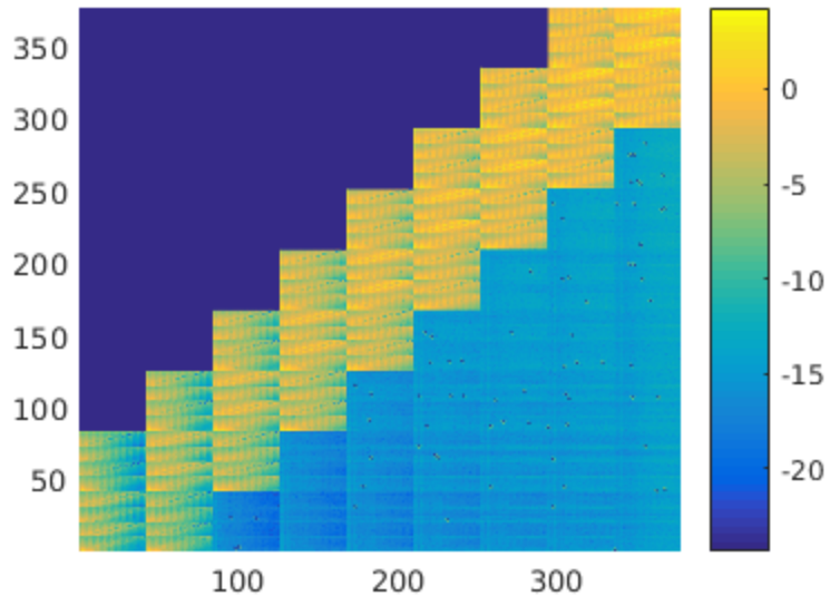
Hessian matrix : \log_{10}(|H|)
