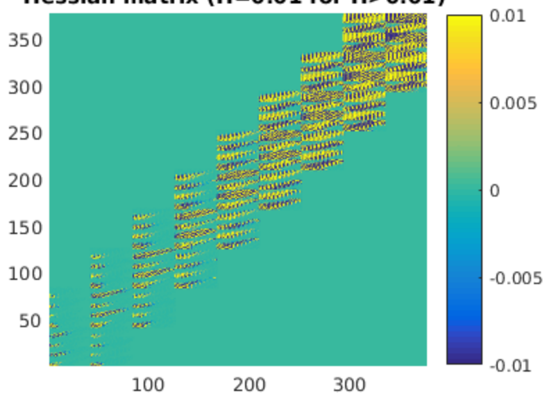
Hessian matrix (H=0.01 for H>0.01)
