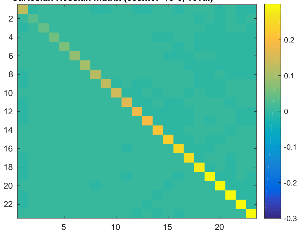
Cartesian Hessian matrix (c05xtol=1e-6, 1eval)
