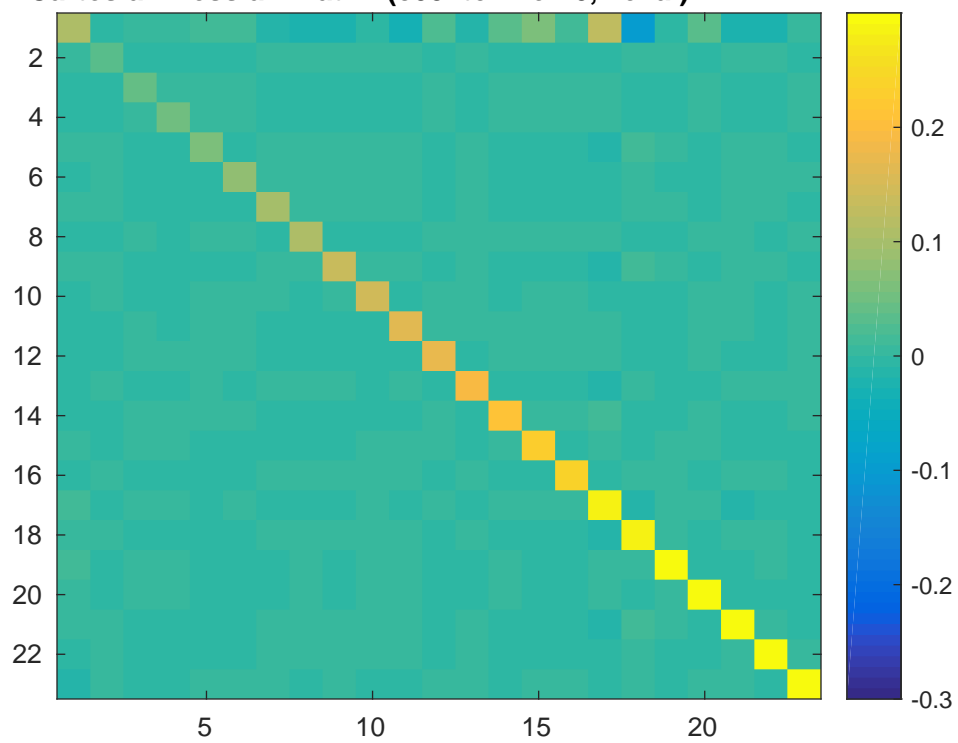
Cartesian Hessian matrix (c05xtol=1e-10, 2eval)
