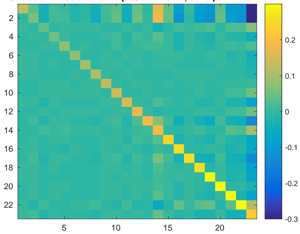
Cartesian Hessian matrix (c05xtol=1e-12, 3eval)
