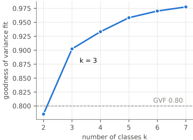
Class-count elbow (Jenks, network CDI)
