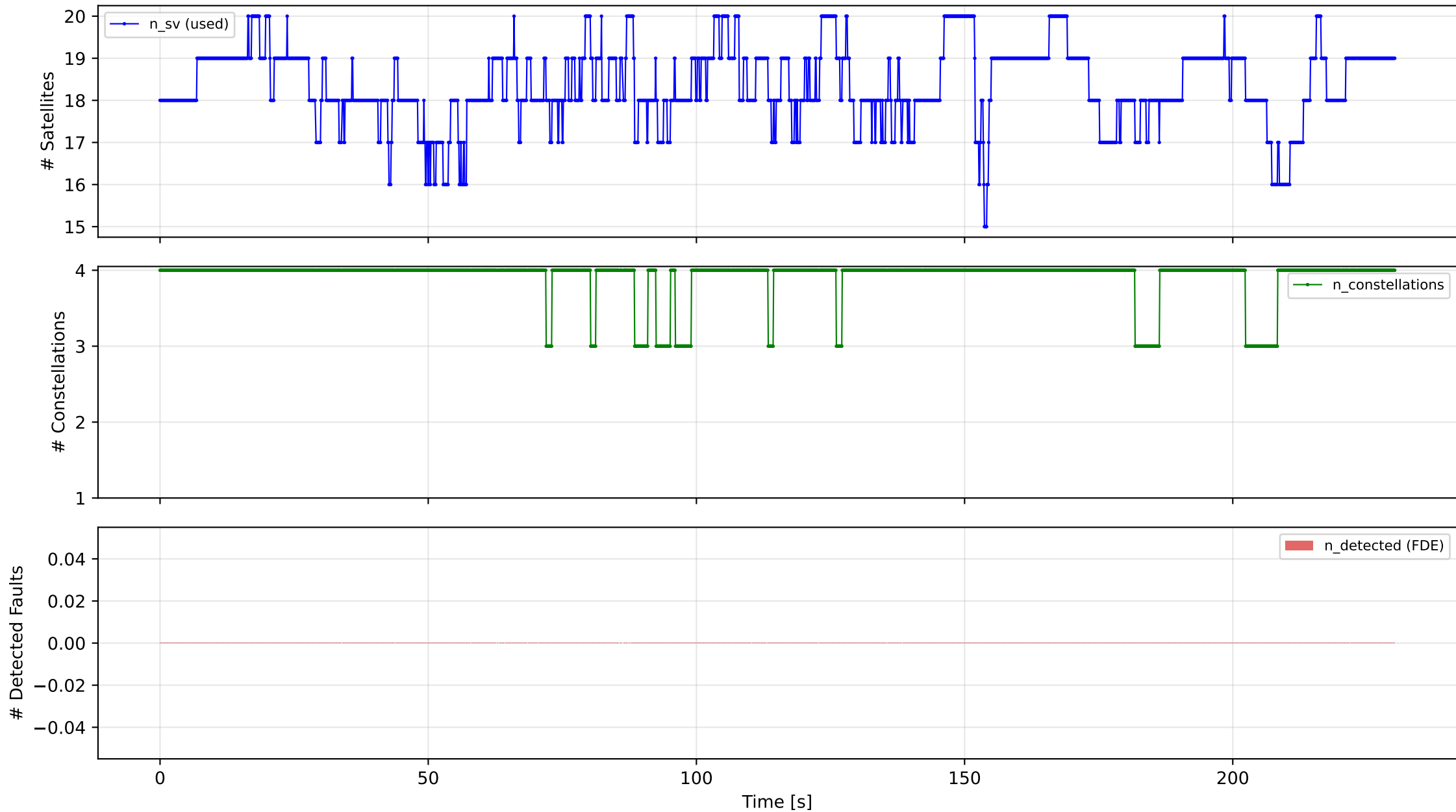
Fig B3 — GNSS Satellite Health Overview
