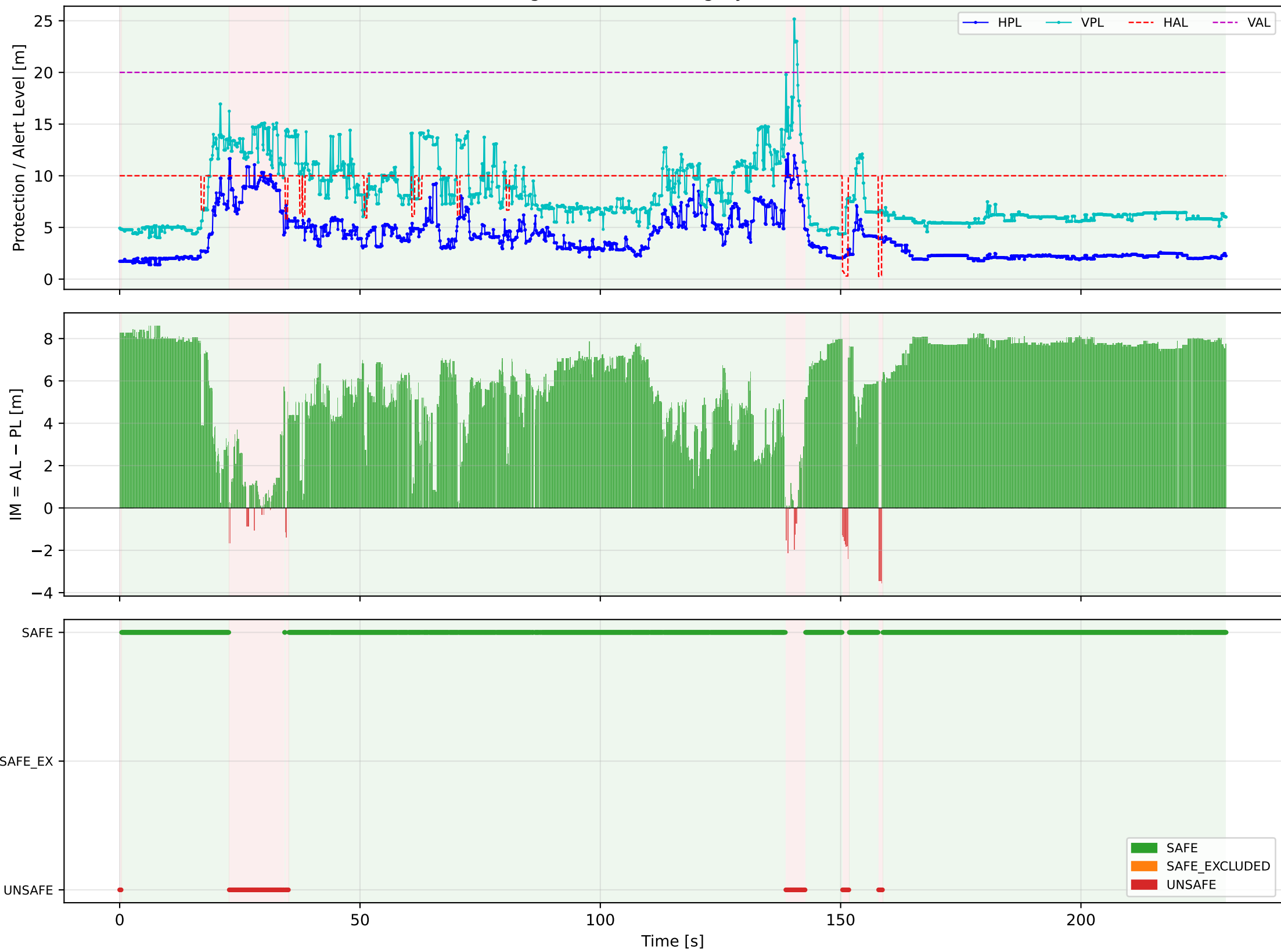
Fig B1 — ARAIM Integrity Timeline
