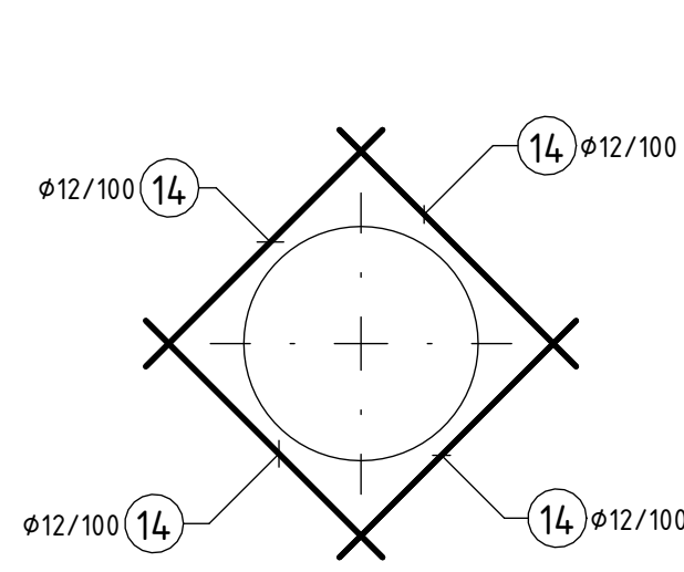
DETAIL 1 1: 25
