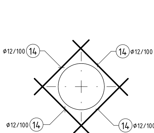
DETAIL 1 1: 25
