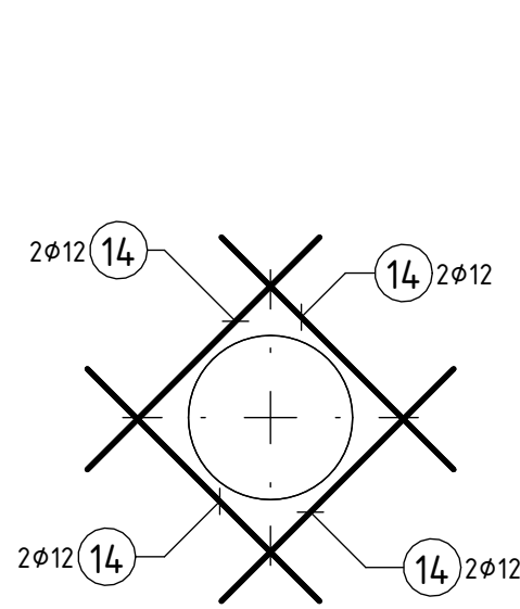
DETAIL 1 1: 25
