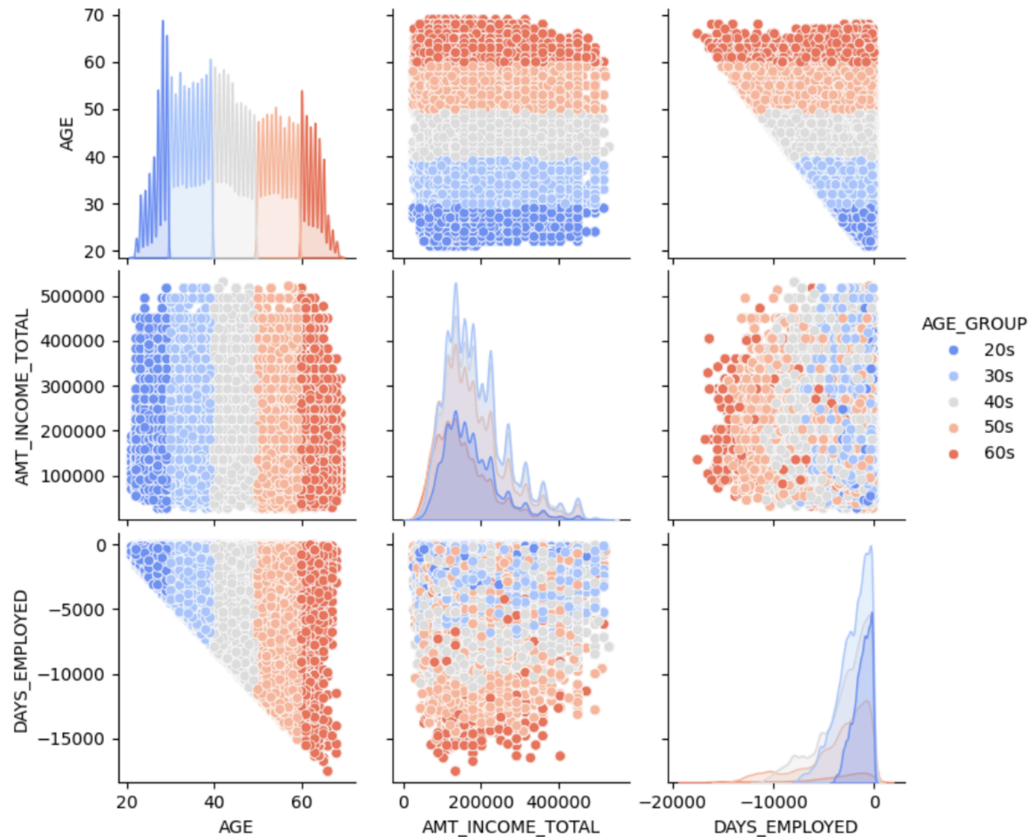
Pair Plot
