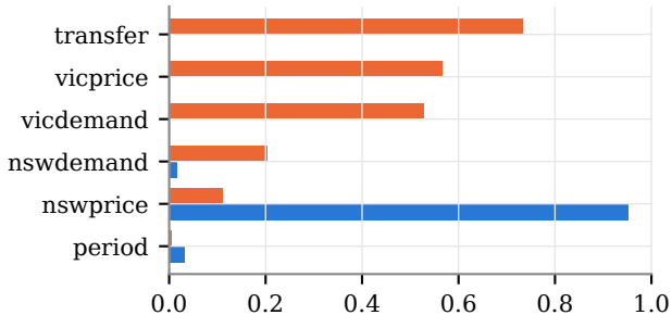
Elec2: time block 0 \rightarrow 7 acc 81.7 \rightarrow 82.4%
