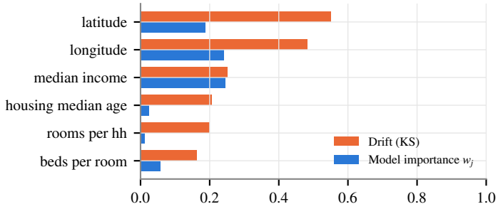
Housing: coastal \rightarrow inland acc 88.4 \rightarrow 61.3%
