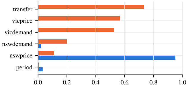
Elec2: time block 0 \rightarrow 7 acc 81.7 \rightarrow 82.4%
