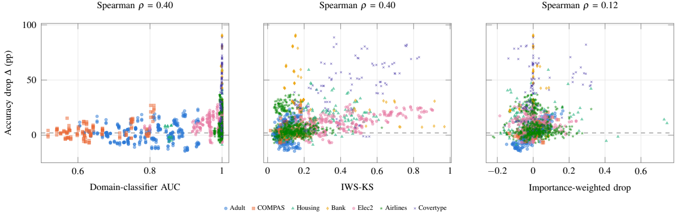
Fig. 2. Accuracy drop versus three signals for every evaluation. The domain-classifier AUC saturates at 1 for most natural shifts, so it cannot rank them; IWS -KS spreads the same pairs out. The density-ratio estimate (right) is close to zero for most harmful pairs because their loss comes from P(Y|X) . Dashed line: harm threshold \tau = 2 pp.
