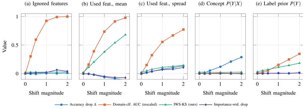
Fig. 3. Synthetic shifts with known ground truth. Data-only drift (orange) reacts to every change in P(X) , harmful or not. IWS (green) ignores irrelevant drift (a) but cannot tell helpful from harmful movement of used features (b, c). No label-free signal sees concept shift (d).
