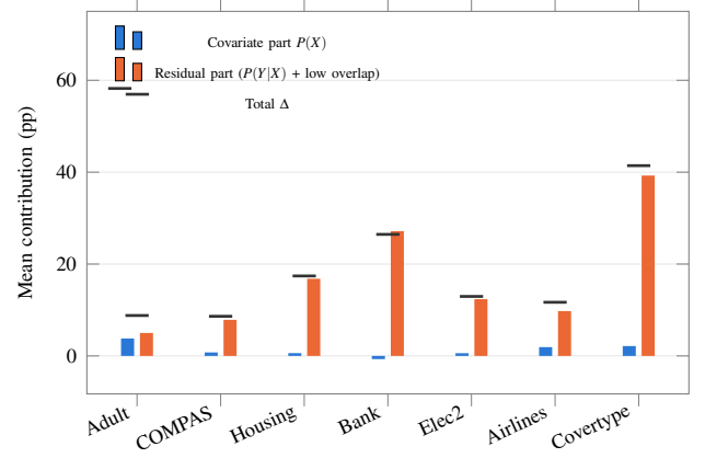
Fig. 5. Mean decomposition of harmful drops (Eq. 4). The residual, conditional part dominates on every dataset.
