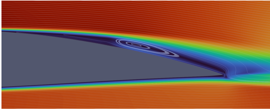
Figure 2: Laminar separation bubble visualized using streamlines
