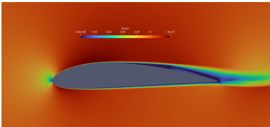
Figure 1: Velocity field as visualized in ParaView
