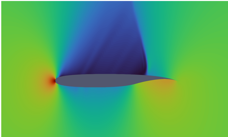
Figure 3: Pressure field as visualized in ParaView
