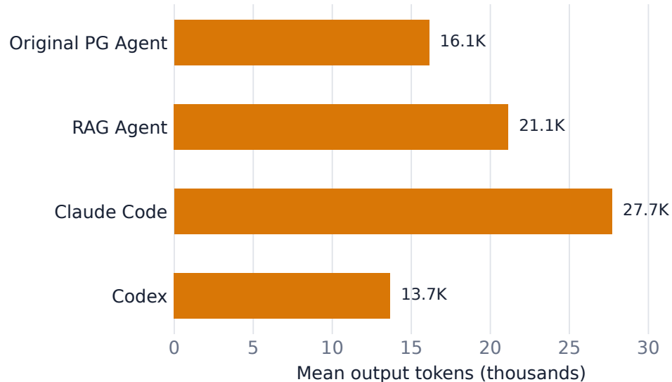
b Mean output tokens
