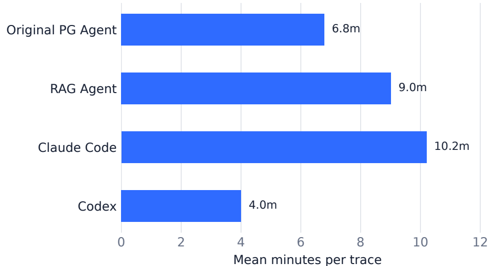
a Mean elapsed time
