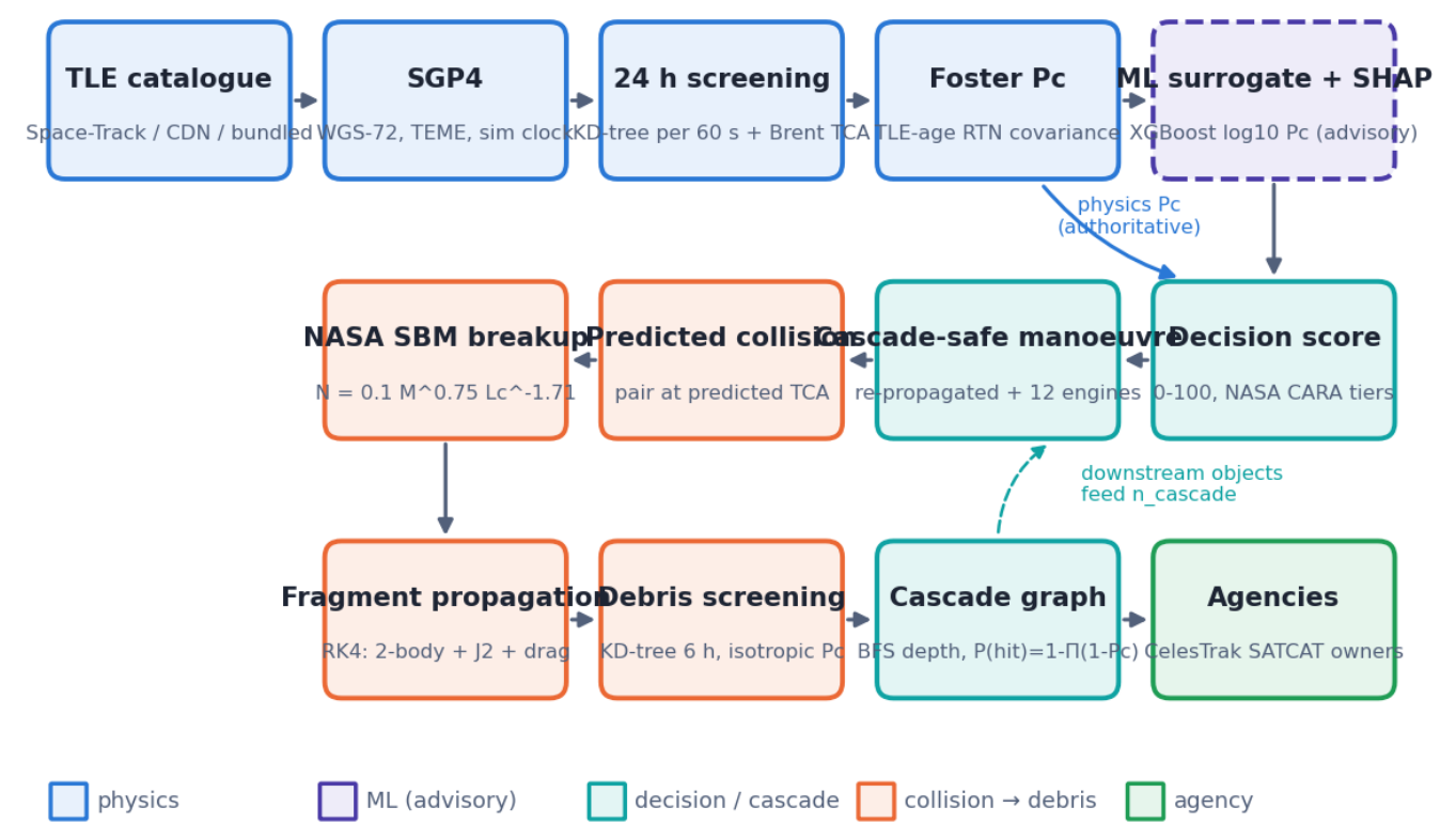
Source: Pipeline as implemented in backend/main.py::refresh_alerts_once and the /api/debris/simulate route (see docs/HOW_IT_WORKS.md for each module). Dashed box: advisory model that never writes the physics Pc.
