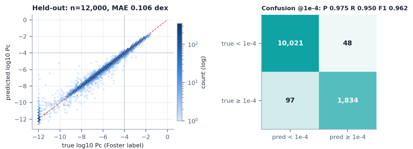
Source: Held-out split regenerated with app.ml.train_risk_surrogate.generate_encounters (seed 20261008, n=60,000, 70/10/20) and scored with the saved risk_model_xgb.json (10 s). Confusion counts match the model card.
