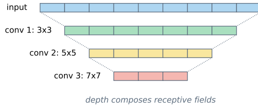
(b) local receptive fields
