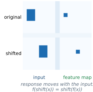
(c) translation equivariance
