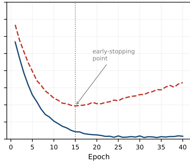
(c) Overfitting
