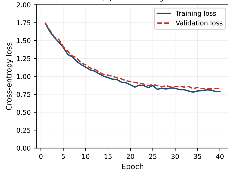
(a) Underfitting
